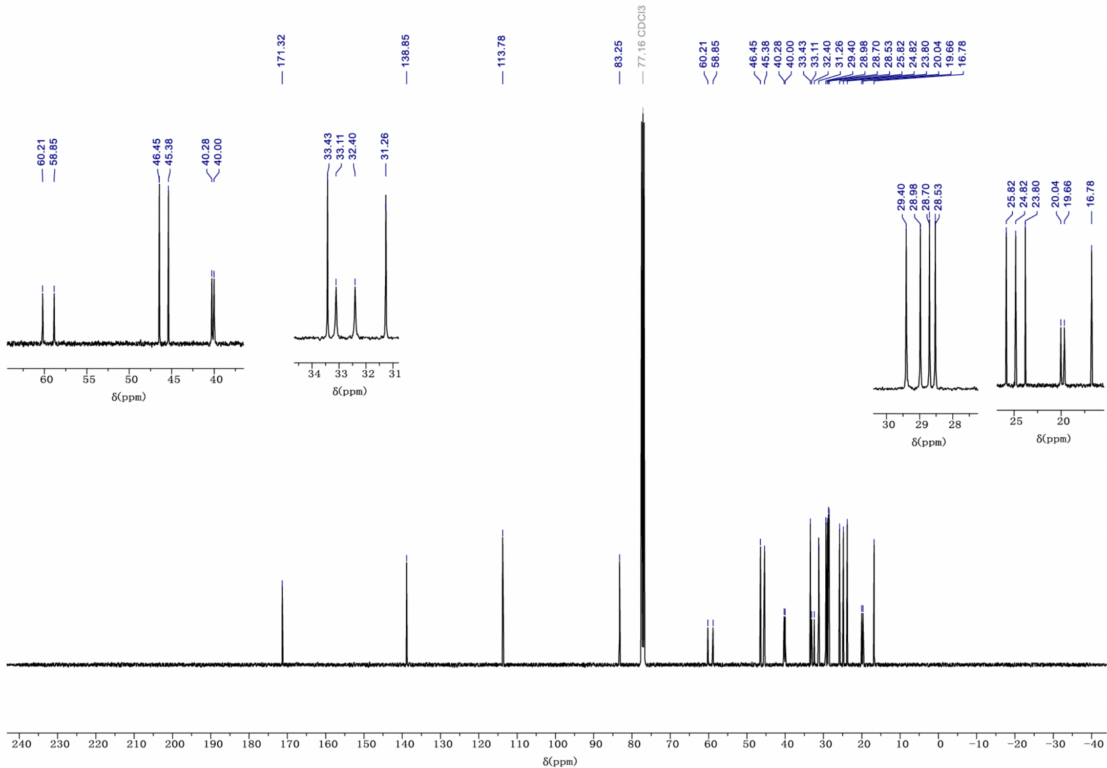
13 C NMR (101 MHz, CDCl 3 ) of compound 2
